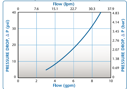
LQ4 Water Flow (0 - 20 GPM)
